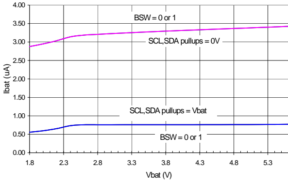
FIGURE 5. I_{BAT} vs V_{BAT} , SIB = 0
