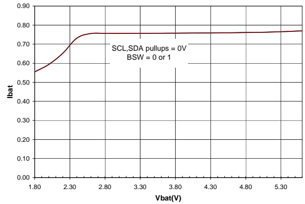
FIGURE 6. I_{BAT} vs V_{BAT} , SIB = 1
