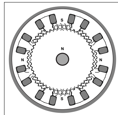
Figure 3. Cross-section of a hybrid stepper motor.
