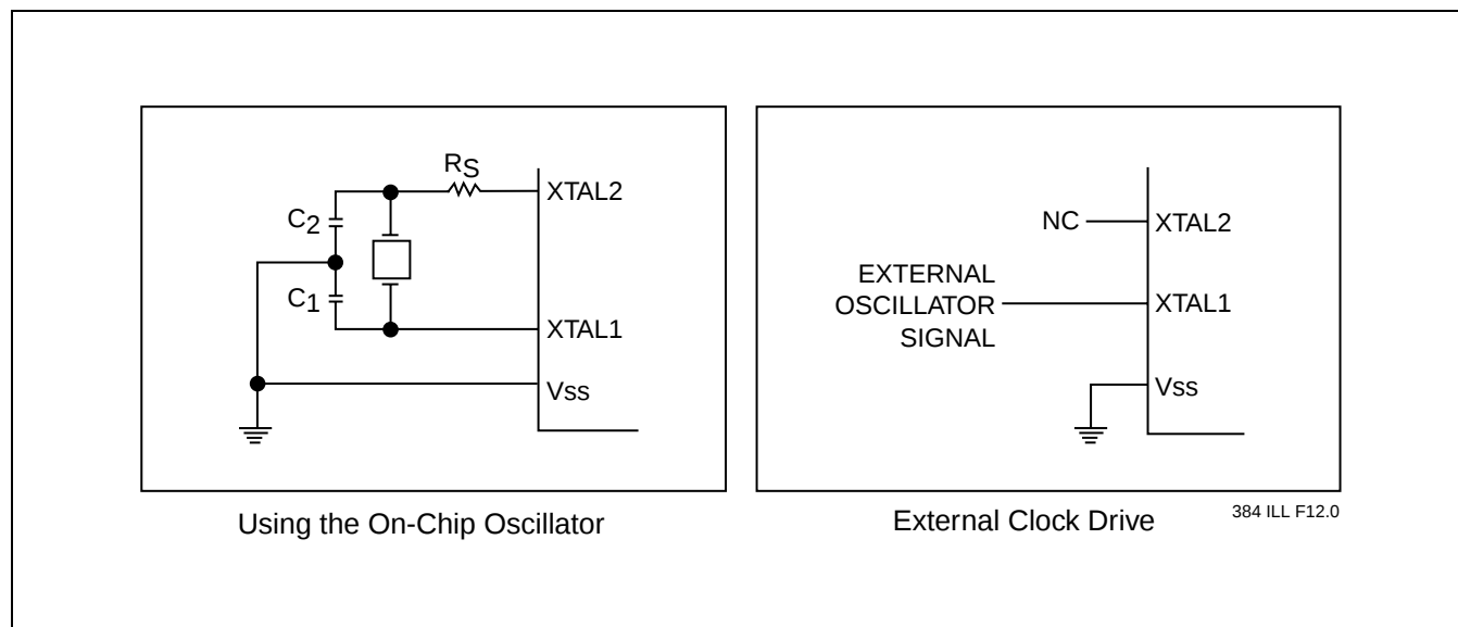
FIGURE 9-2: OSCILLATOR CHARACTERISTICS
