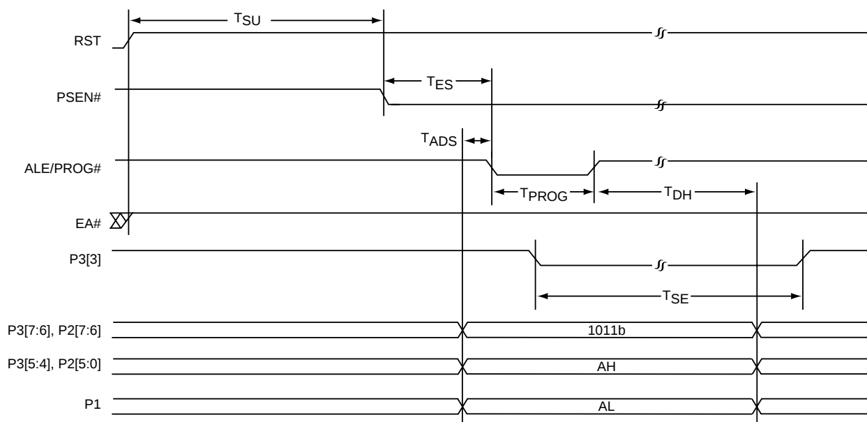
FIGURE 4-7: SECTOR-ERASE
