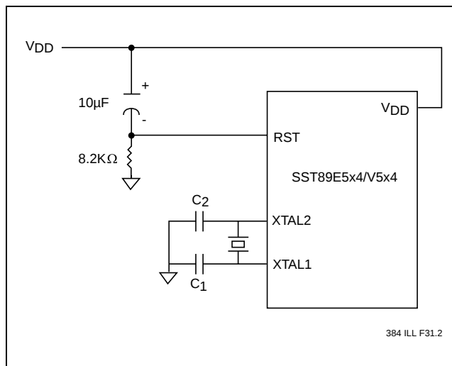
FIGURE 9-1: POWER-ON RESET CIRCUIT
