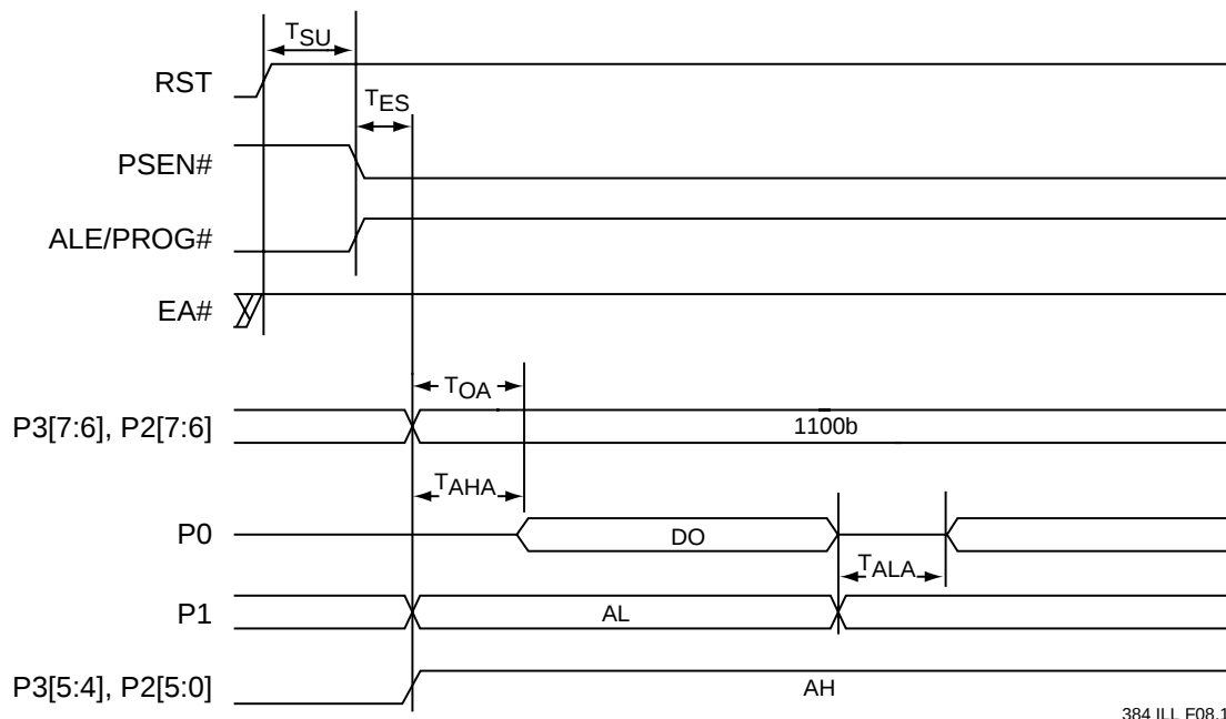
FIGURE 4-11: BYTE-VERIFY
