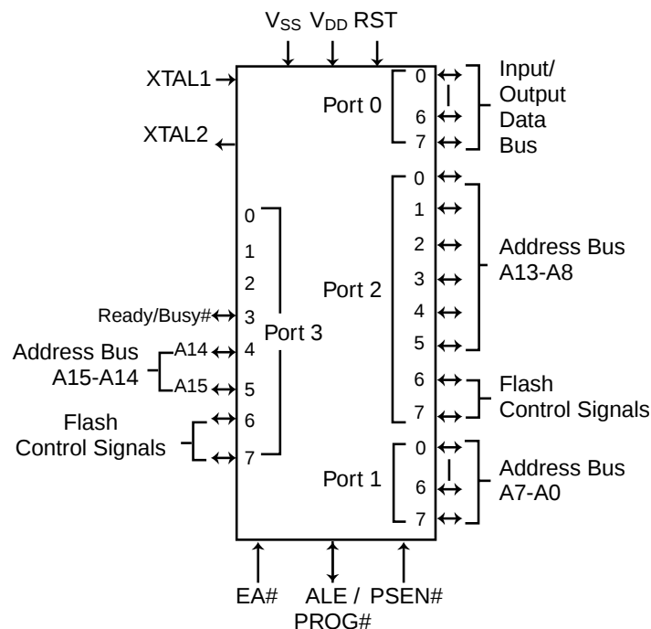
FIGURE 4-1: I/O PIN ASSIGNMENTS FOR EXTERNAL HOST MODE
