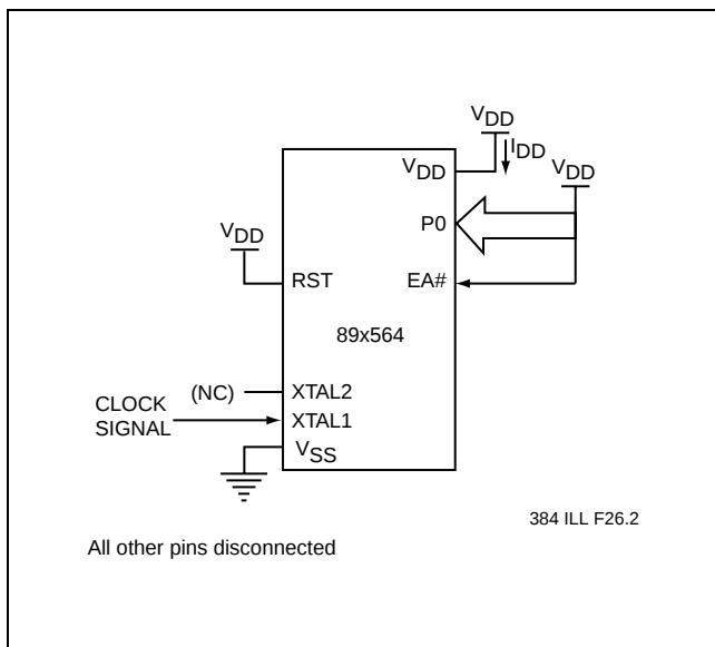
FIGURE 10-1: I_{DD} TEST CONDITION, ACTIVE MODE
