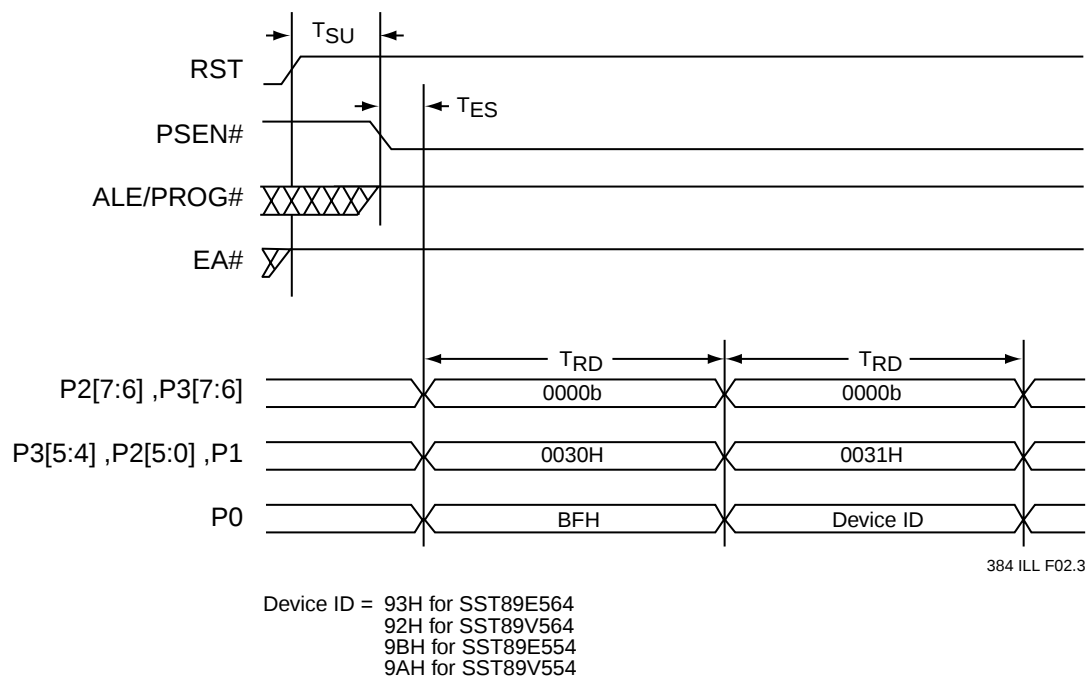
FIGURE 4-2: READ-ID
