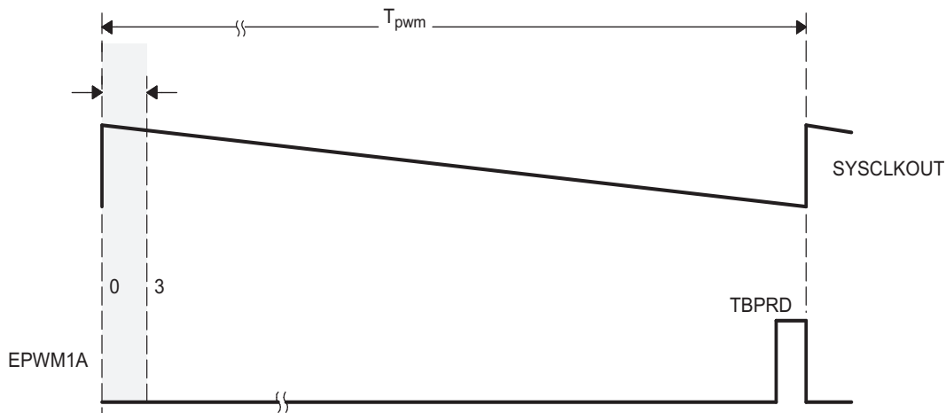
Figure 8. High % Duty Cycle Range Limitation Example ( \text{HRPCTL}[\text{HRPE}] = 0 )
