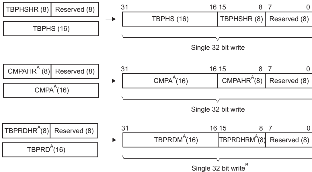
Figure 3. HRPWM Extension Registers and Memory Configuration
