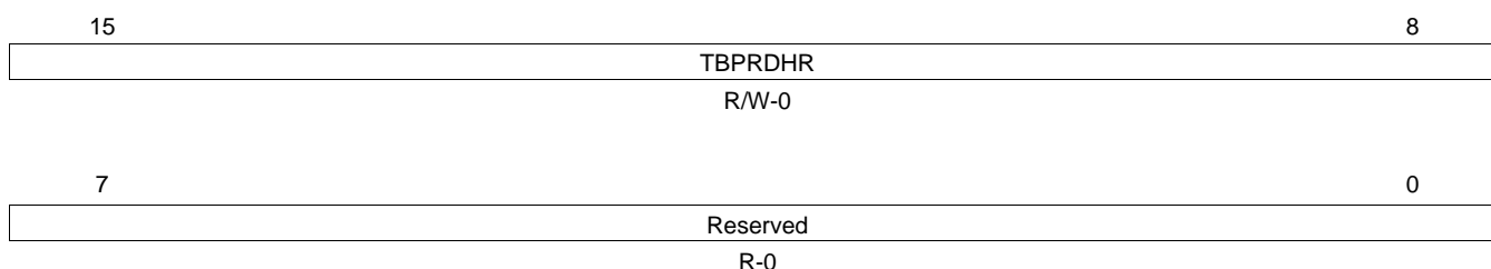
Figure 20. Time-Base Period High Resolution Mirror Register
