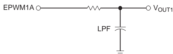
Figure 13. Simple Reconstruction Filter for a PWM Based DAC
