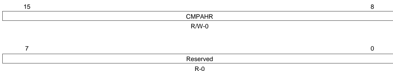
Figure 19. Compare A High Resolution Mirror Register
