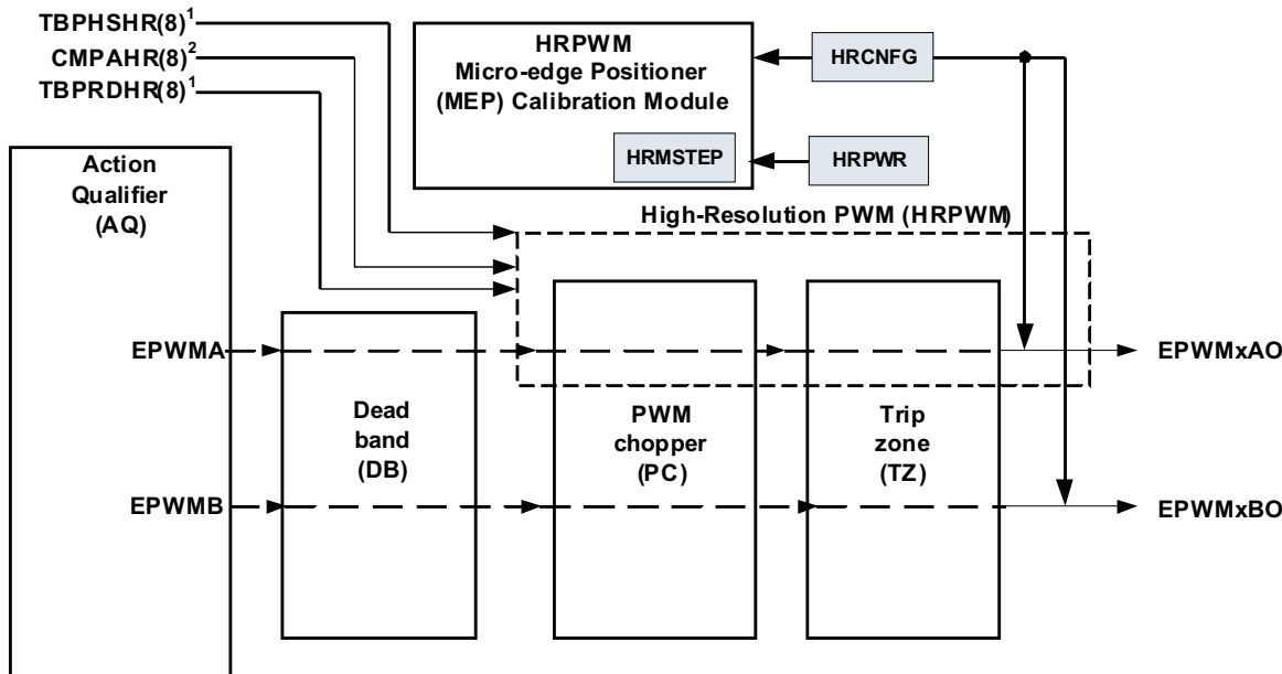
Figure 5. HRPWM Block Diagram
