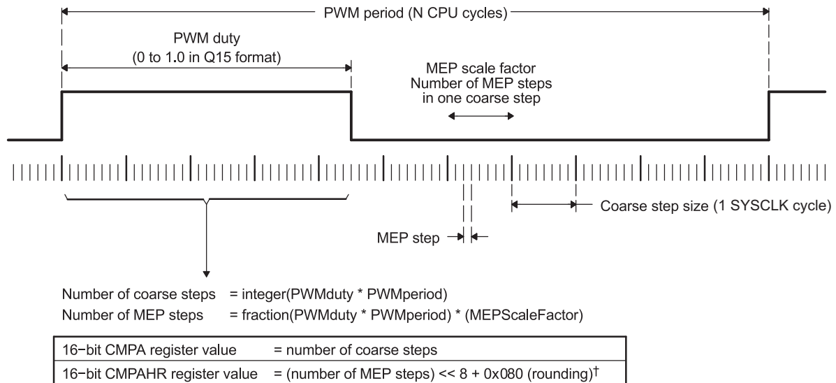
Figure 2. Operating Logic Using MEP
