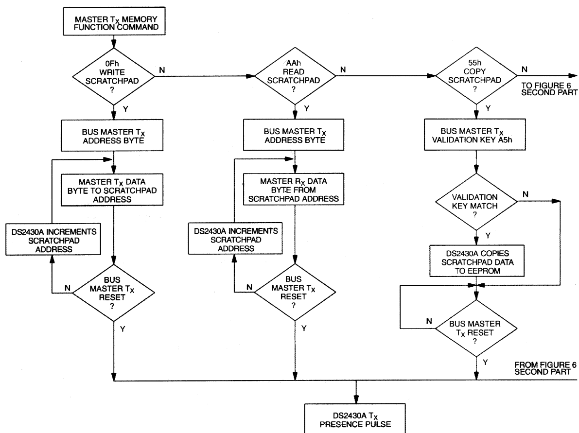
MEMORY FUNCTION FLOW CHART Figure 6
