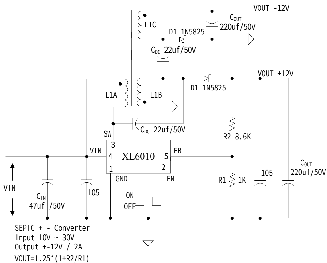
Figure9. XL6010 Typical System Application (SEPIC Inverting Converter)
