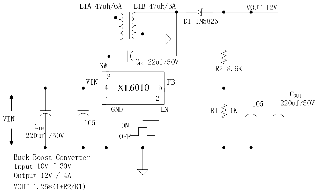
Figure6. XL6010 Typical System Application (SEPIC Buck-Boost Converter)
