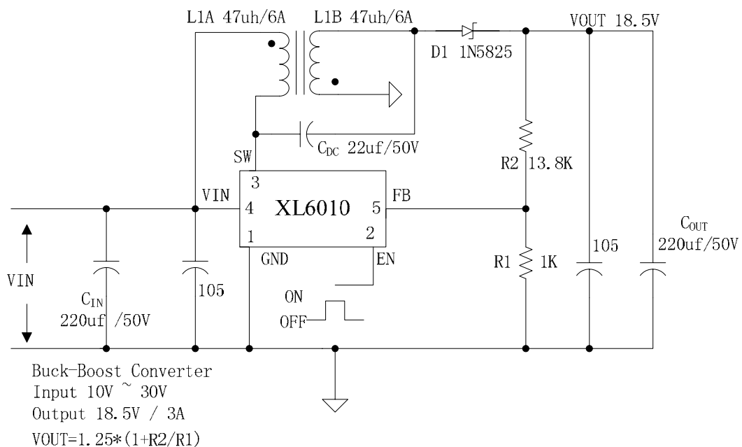
Figure7. XL6010 Typical System Application (SEPIC Buck-Boost Converter)
