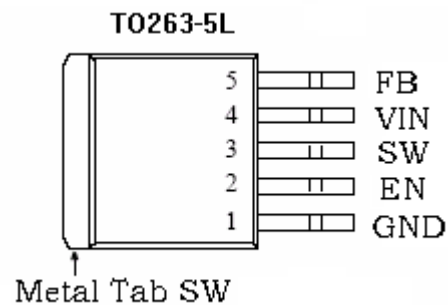
Figure2. Pin Configuration of XL6010 (Top View)
