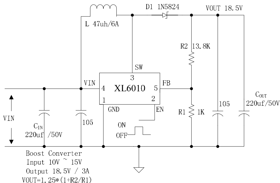
Figure4. XL6010 Typical Application Circuit (Boost Car Adapter)
