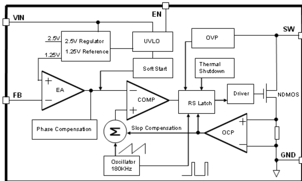
Figure3. Function Block Diagram of XL6010
