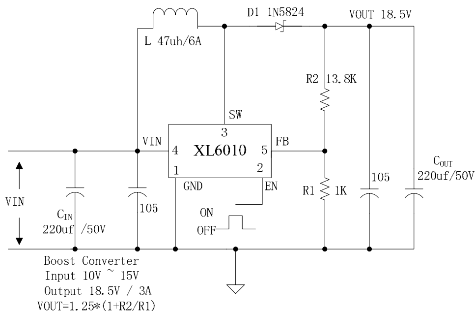
Figure5. XL6010 Typical System Application (Boost Car Adapter)
