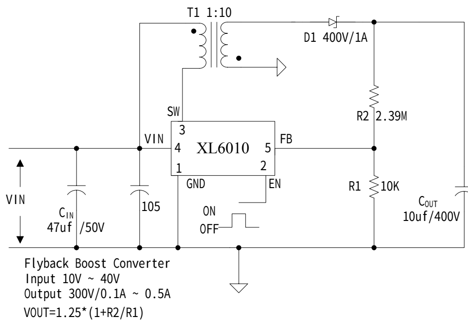
Figure8. XL6010 Typical System Application (Flyback Boost Converter)
