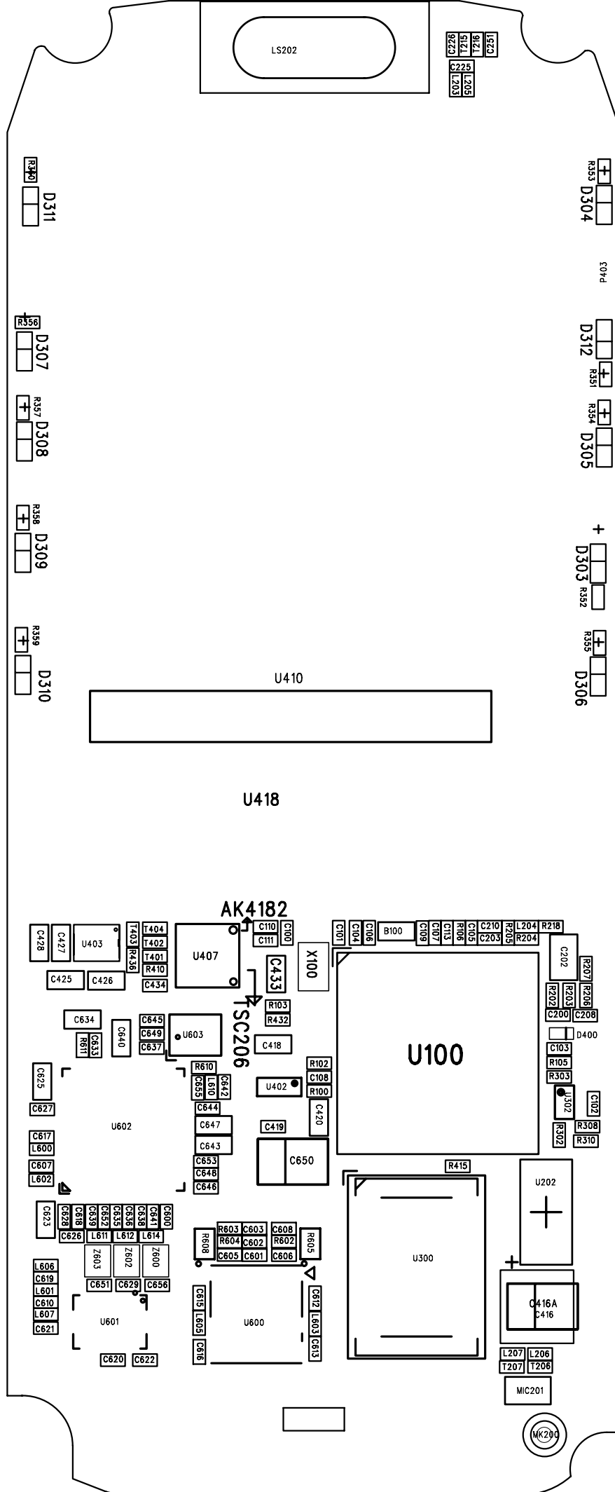
V2.0 Assembly TOP
