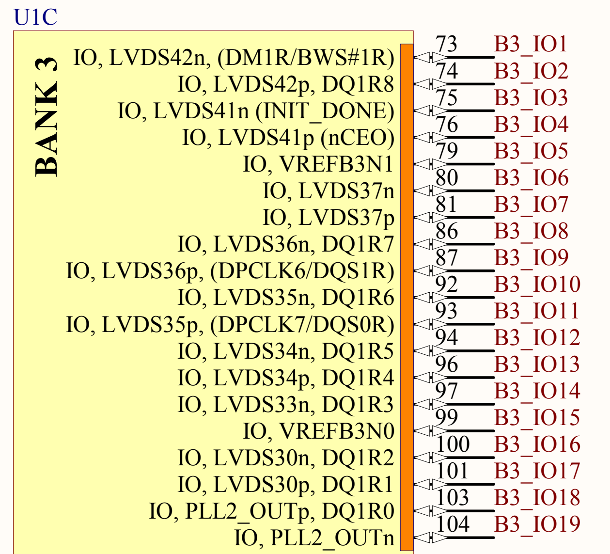
EP2C5T144C6
