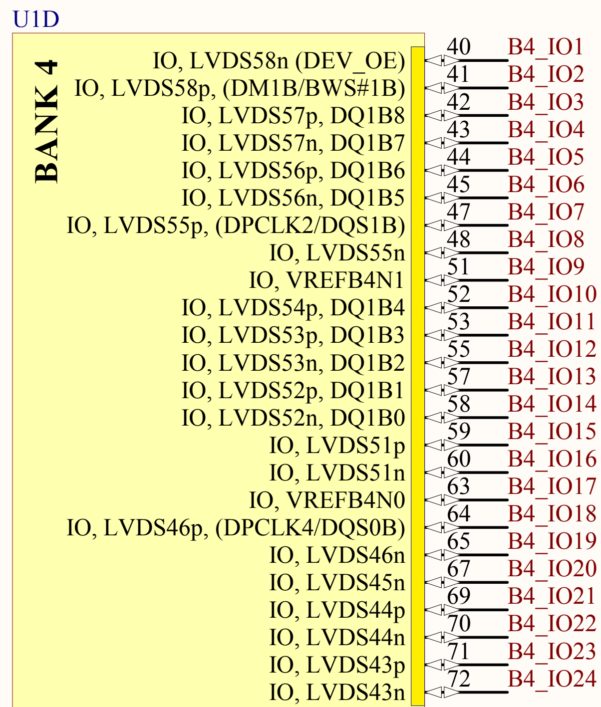
EP2C5T144C6
