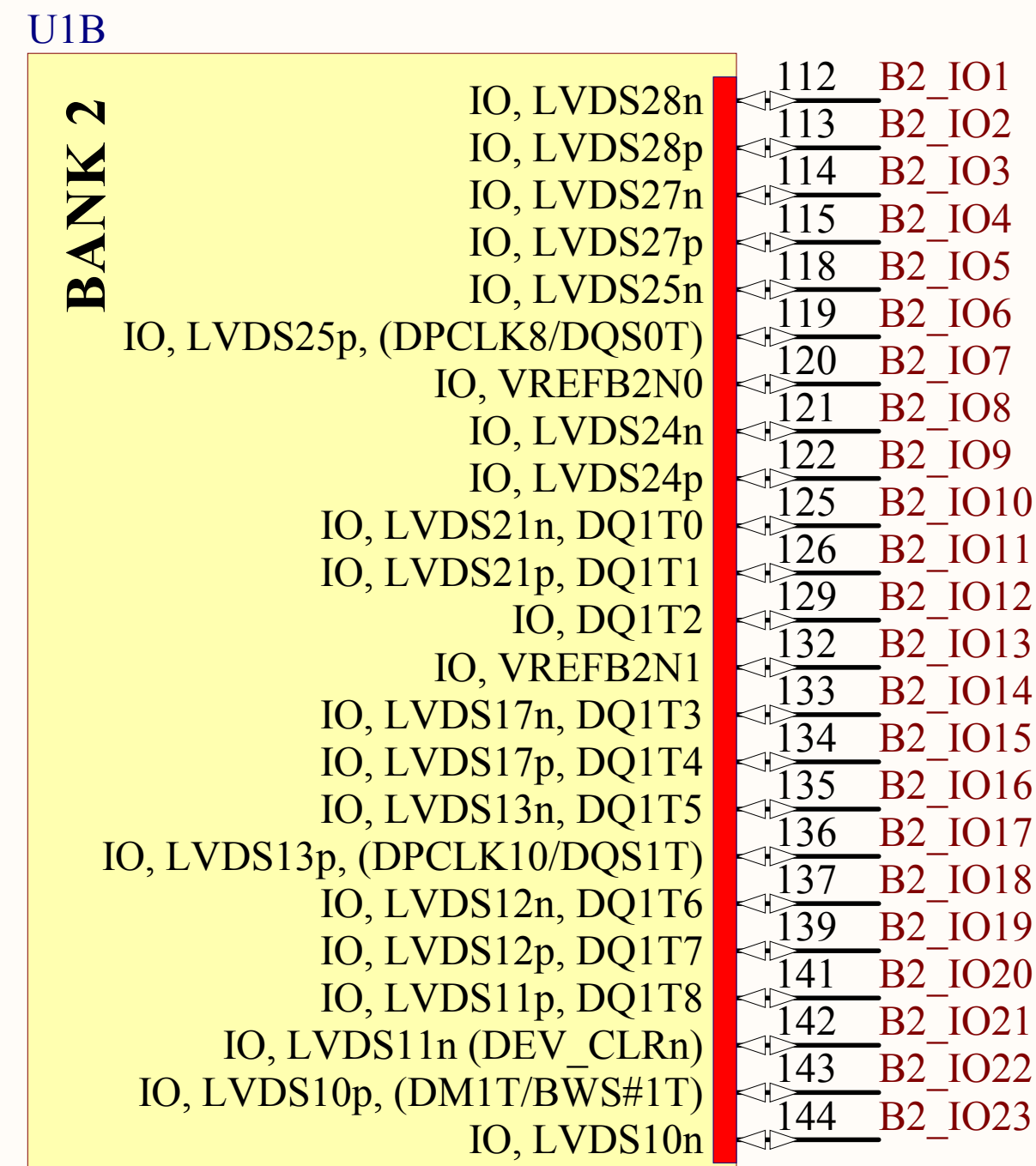
EP2C5T144C6
