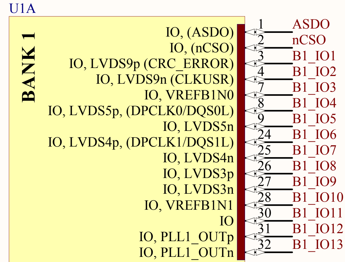
EP2C5T144C6
