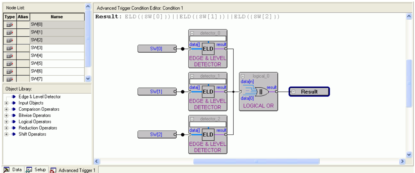
Figure 20. Arrange the elements to create a circuit that looks like this.
