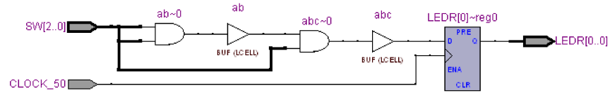
Figure 25. The circuit implemented by the code in Figure 24
