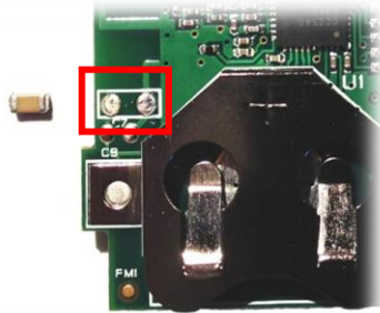
Figure 5- Capacitor C7 Removed
