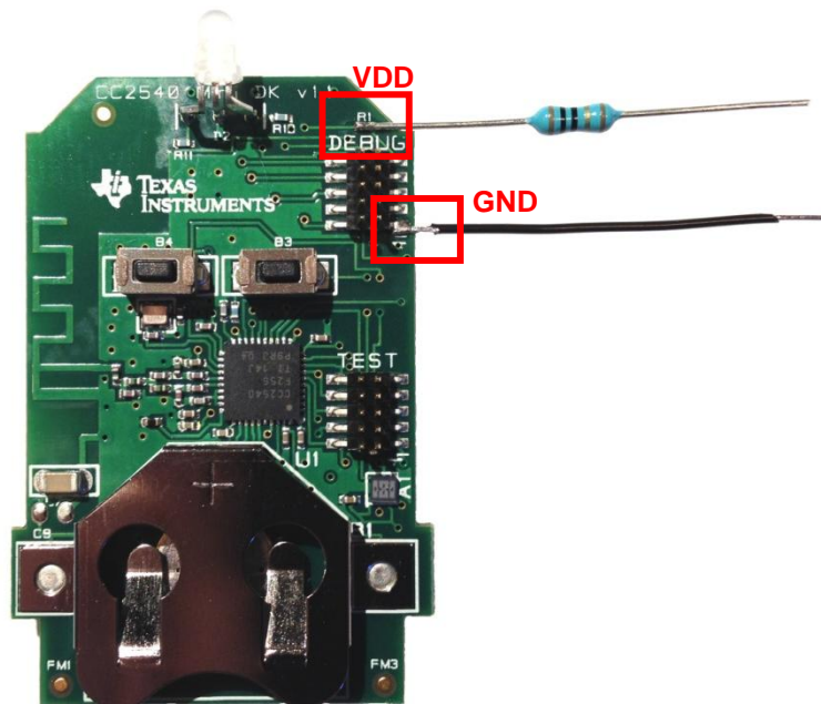
Figure 4- 10 Ω Resistor Soldered in Line with VDD
