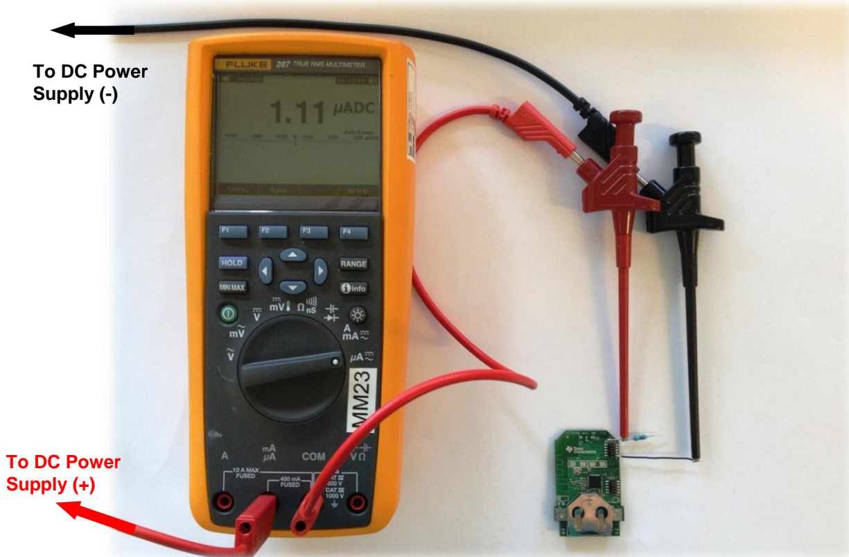
Figure 17- 1 μA PM2 Sleep Current Measured on Keyfob
