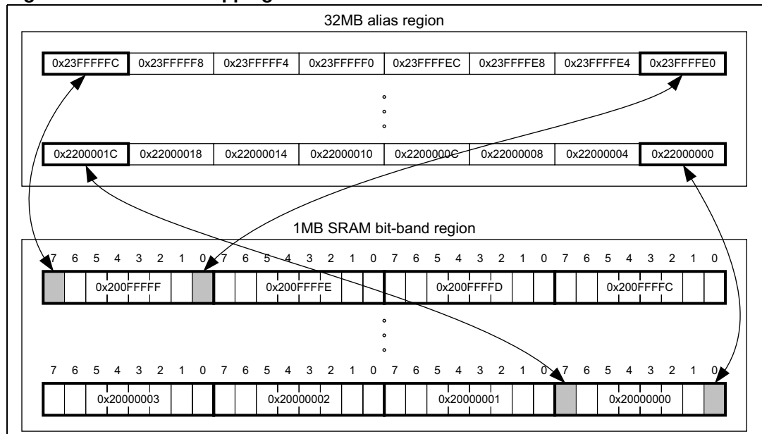
Figure 10. Bit-band mapping
