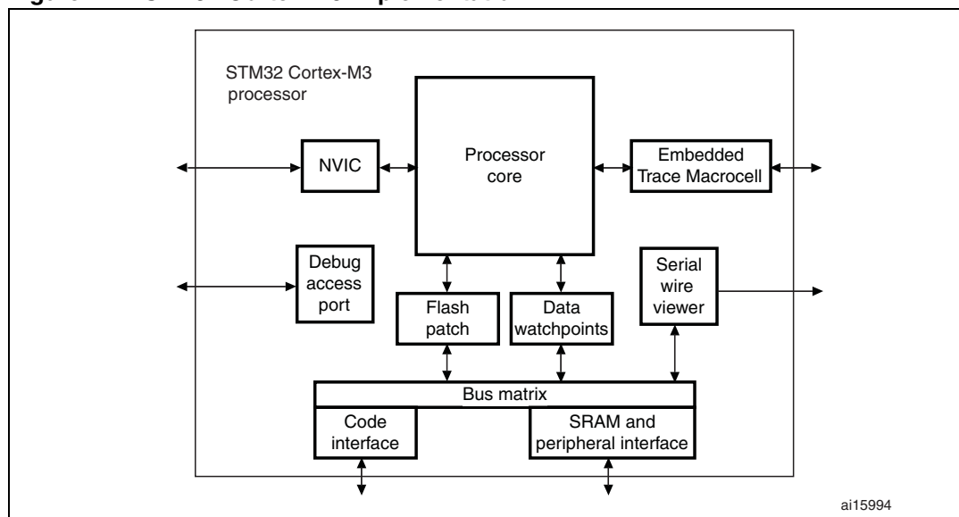
Figure 1. STM32 Cortex-M3 implementation
